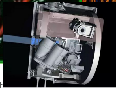
Fig.2: Cut through the LUCI cryostat. The pink area indicates the location of the MOS-unit
